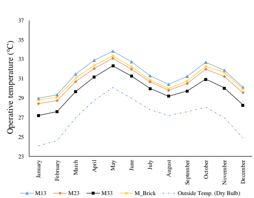
Fig 7. Differences in the operative temperature with respect to different wall materials and 6 mm clear window glass with blue tint.
